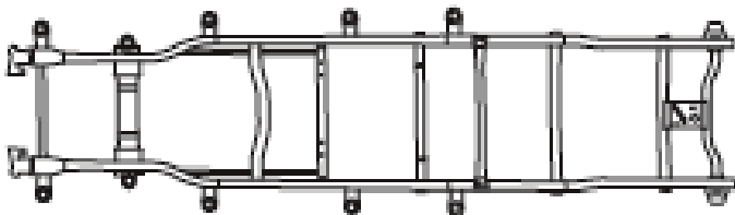
UNDERBODY VIEW
